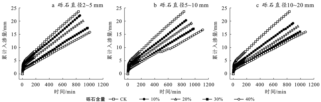
图 3 不同砾石含量及粒径下累积入渗量变化 Fig.3 Variation of cumulative infiltration under different gravel content and particle sizes
